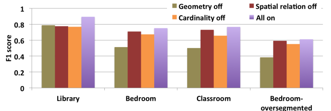
Figure 12: Impact of individual energy terms on object classification. Each energy term contributes to the overall performance in each dataset.
